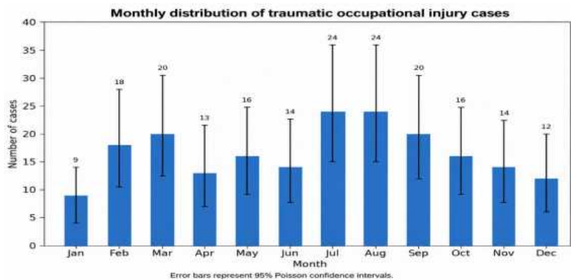
Figure -1. Monthly distribution of traumatic occupational injury cases with exact case numbers on bars and 95% Poisson confidence interval error bars. The y-axis shows the number of cases and the x-axis shows calendar month. May-July had two observed years, while the remaining months had three observed years during the study period.
